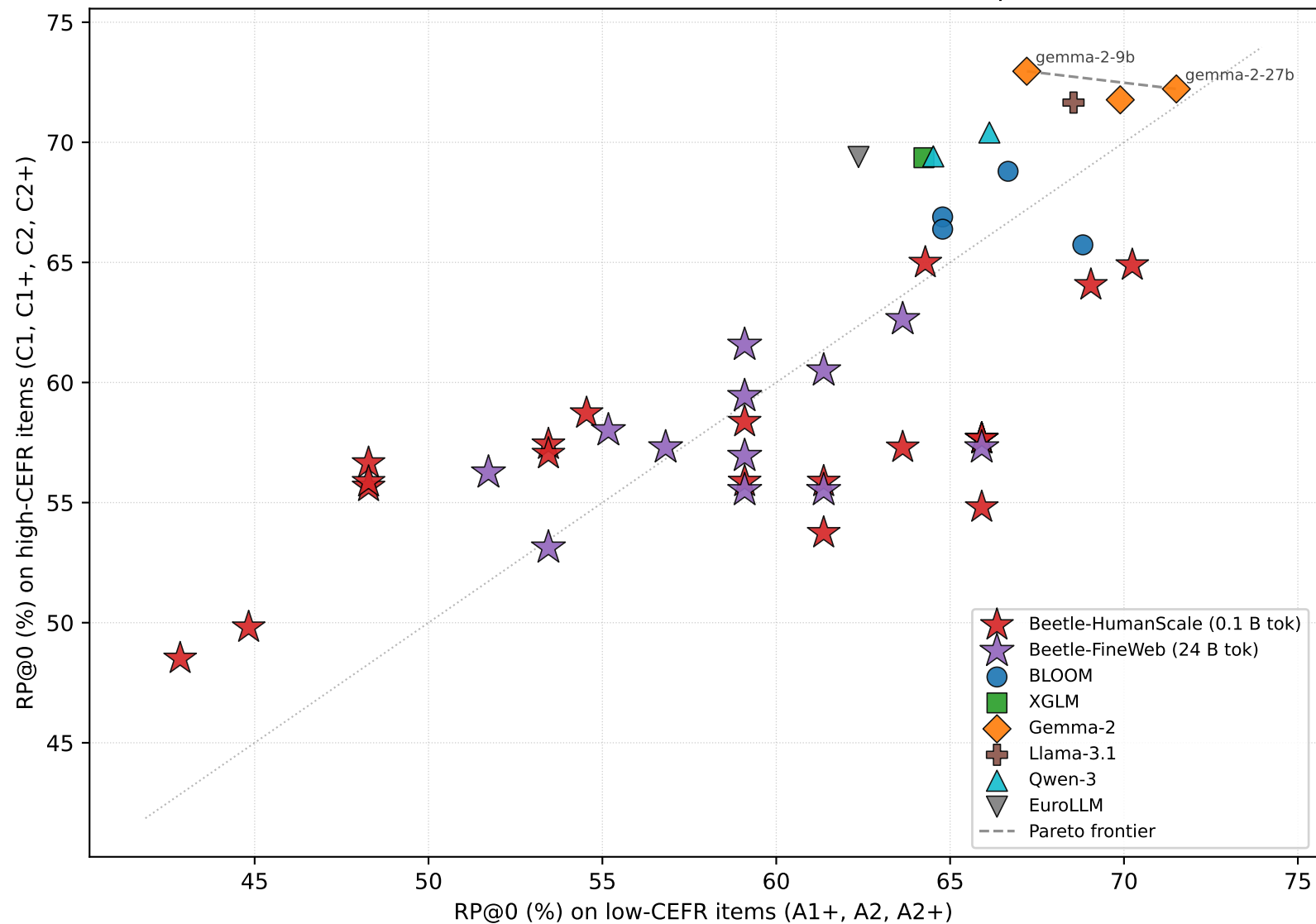
BLISS CEFR Pareto: which models match low- vs high-proficiency learners? (L1 \in {Dutch, German, Chinese} for fair Beetle comparison)
